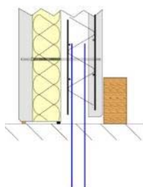
Figure 89 - Calage ≥ 30 mm
